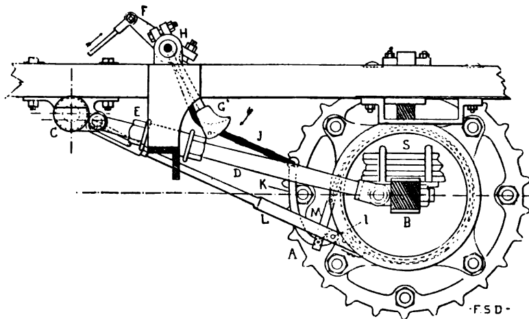
Fig. 454.—The Hub Brake and Operating Levers Used on the Panhard Carriages.—The arm, F, being pushed in the direction of the arrow, causes the arm, G, on the same pivot, H, to move in the opposite direction, as indicated by the lower arrow. Through this arm, G, runs the cable, J, as shown, which, pulling on the arm, K, pivoted at I, pulls the strap, shown by dotted lines around the drum, S. The other end of the strap attached to the short arm of the lever, K, is thus drawn toward the same point, a tight frictional bind being the result.
